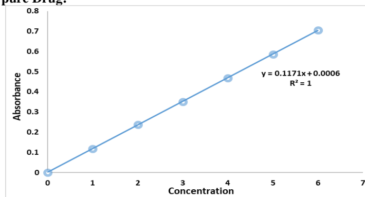
Figure.No .3 Standard calibrationcurve of Macitentan in 0.1N HCl buffer
